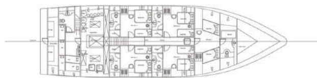
LOWER DECK
